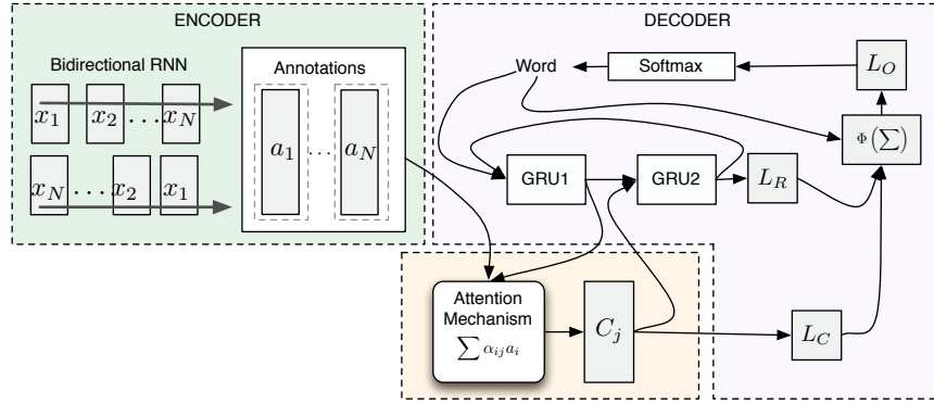
Fig. 1. Attention-based NMT system
