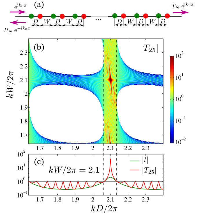
FIG. 5. (a) Finite periodic case with N cells, green(red) is a scatterer with loss (gain). (b) Transmission coefficient as a function of kD and kW for N = 25 . White regions correspond to band gaps. (c) Transmission for kW/2\pi = 2.1
