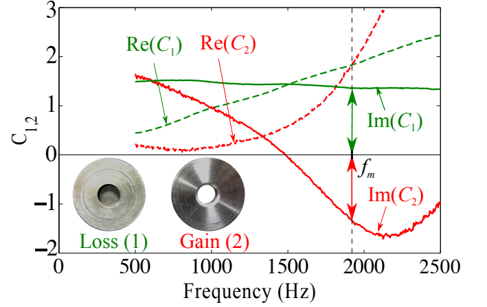
FIG. 2. Real and imaginary part of the measured impedance parameters C_1 and C_2 . When the imaginary part of C_2 is negative the diaphragm get some gain. At the frequency f = f_m , gain and loss are balanced C_2 = C_1^* .
