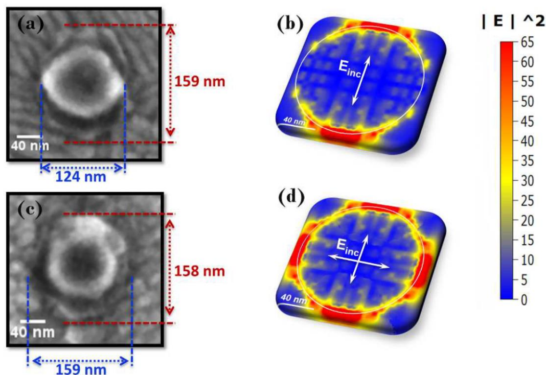
Fig. 3 SEM images of a single nanoparticle after plasmon-induced grafting of (a) carboxyphenyl layers along the Y direction and (c) additional hydroxyethyl phenyl layers along the X axis. Irradiation conditions: \lambda_{inc} = 633 nm, 180 seconds with a power of P=0.8 mW \mu\text{m}^{-2} . Mapping of the near-field intensity enhancement |E|^2 upon irradiation along the Y axis (b) and both X and Y axis (d), on a unit cell with a nanodisk of 100 nm diameter, H = 50 nm, using the DDA method.
