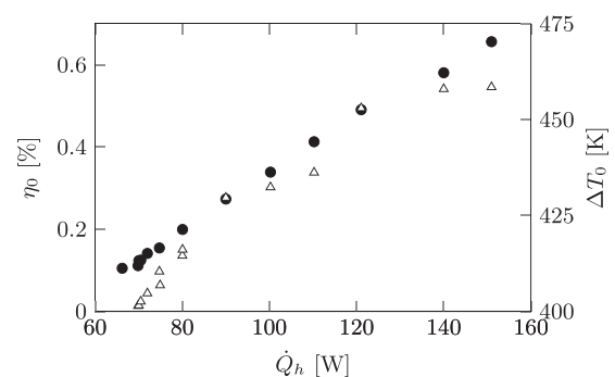
FIG. 2. Overall efficiency \eta_0 ( \bullet ) of the engine and temperature difference \Delta T_0 ( \Delta ) through the regenerator when the auxiliary source is not powered, for various input heat powers \dot{Q}_h above the onset threshold. The drive ratio (ratio of the amplitude of the acoustic pressure measured by the microphone \mu to the static pressure P_0 ) varies correspondingly from 1% to 3.2%. These are the reference efficiency and temperature difference for the later comparison with the effect of the active control loop.
