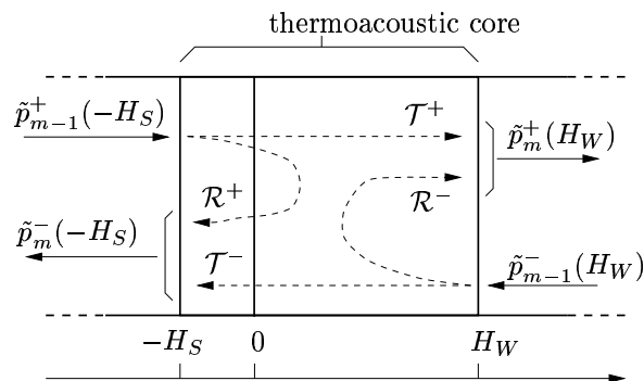
Figure 2: Reflected and transmitted waves at the edges of the thermoacoustic core
