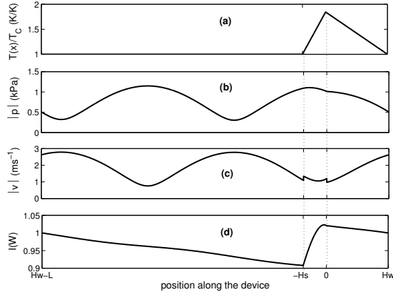
Figure 3: Distribution of the acoustic pressure |\tilde{p}(x)| (b), acoustic velocity |\tilde{v}(x)| (c), and acoustic intensity I = (1/2)Re(\tilde{p}\tilde{v}^*) (d) in the whole device, at threshold for the case of the linear temperature distribution profile (a).
