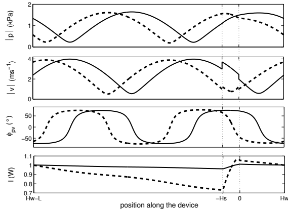
Figure 5: Distribution of the acoustic pressure |\tilde{p}(x)| , acoustic velocity |\tilde{v}(x)| , phase shift \Phi_{pv} and acoustic intensity I = 1/2\text{Re}(\tilde{p}\tilde{v}^*) in the whole device, at threshold for the case of the linear temperature distribution profile. Solid line : \delta_{\kappa}/D_S = 0.1 , dashed line : \delta_{\kappa}/D_S = 0.73 .
