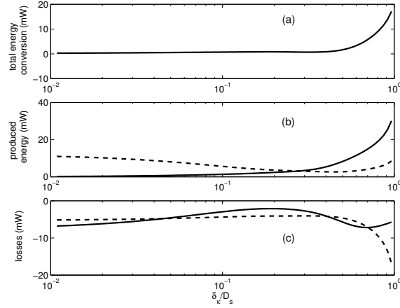
Figure 6: Energy conversion in one stack channel versus \delta_{\kappa}/D_S at threshold condition ( \alpha = 0 ). (a) Total energy conversion. (b) Standing wave component W_{SW} (dashed line) and travelling wave component W_{TW} (solid line) of the produced energy. (c) Viscous component W_{\nu} (dashed line) and thermal component W_{\kappa} (solid line) of the losses.
